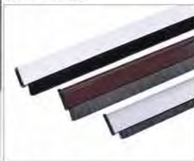
NO: DBLK-15 Adjustable Bottom Brush Seal 1000mm*123mm*8mm-Aluminum alloy Glue
